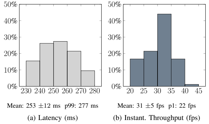
Fig. 4: Observe_{ab} Measurements
