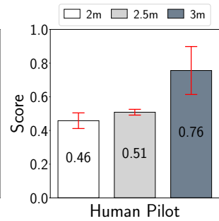
Fig. 17: Human Pilot
