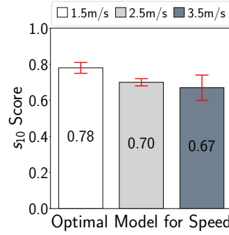
Fig. 28: Baseline Scores
