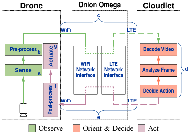
Fig. 2: Detailed View of Our OODA Loop
