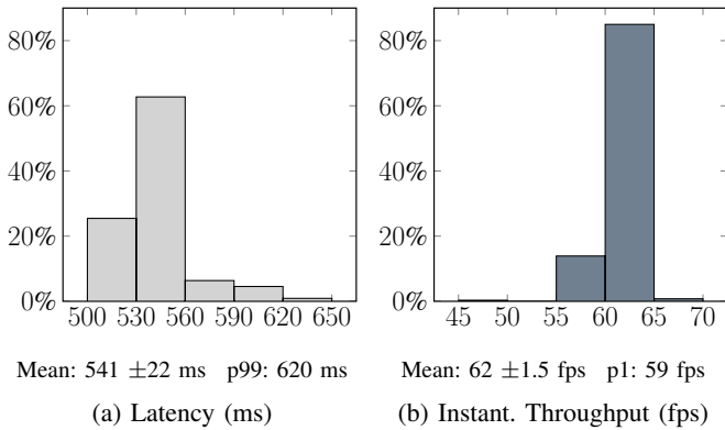
Fig. 6: Original FFmpeg-based Stage-1 Performance
