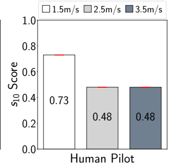
Fig. 29: Human Pilot
