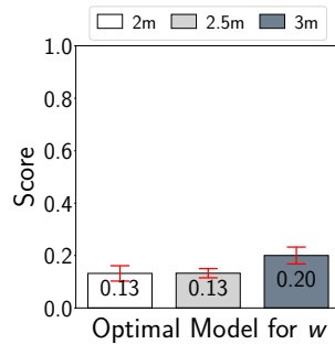
Fig. 16: Baseline Scores
